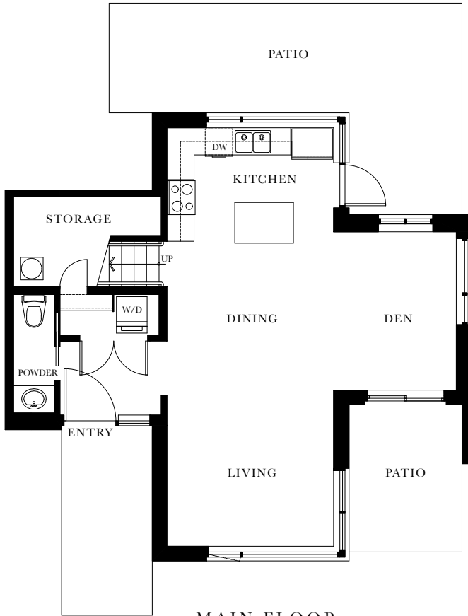
MAIN FLOOR
