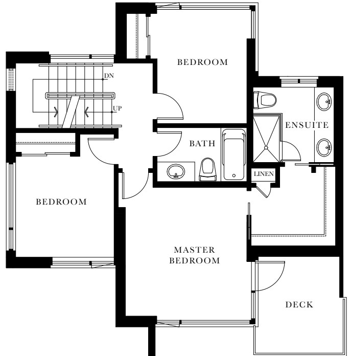
UPPER FLOOR
