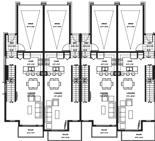
MAIN FLOOR
