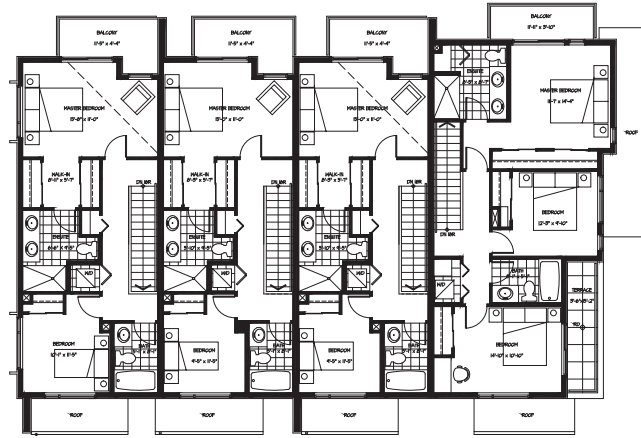
UPPER FLOOR
