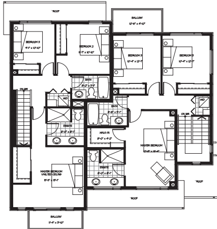
UPPER FLOOR
