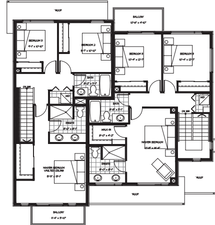
UPPER FLOOR
