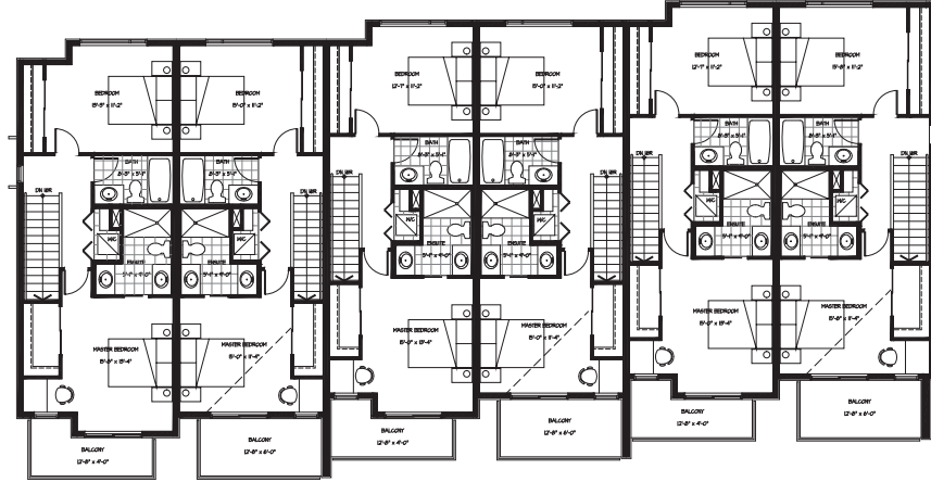
UPPER FLOOR
