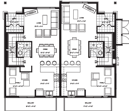
MAIN FLOOR
