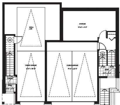
BASEMENT
